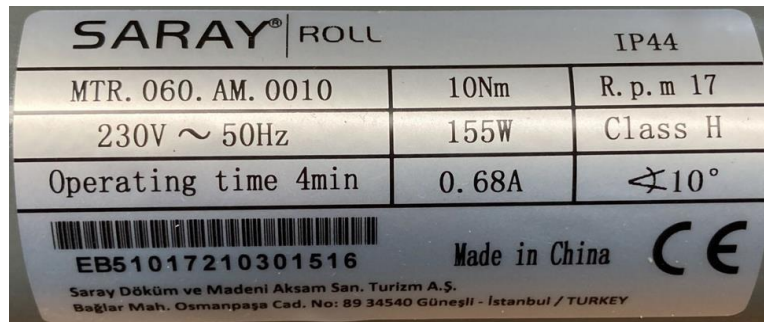
Photo 5. Shutter motor label (remote control)
